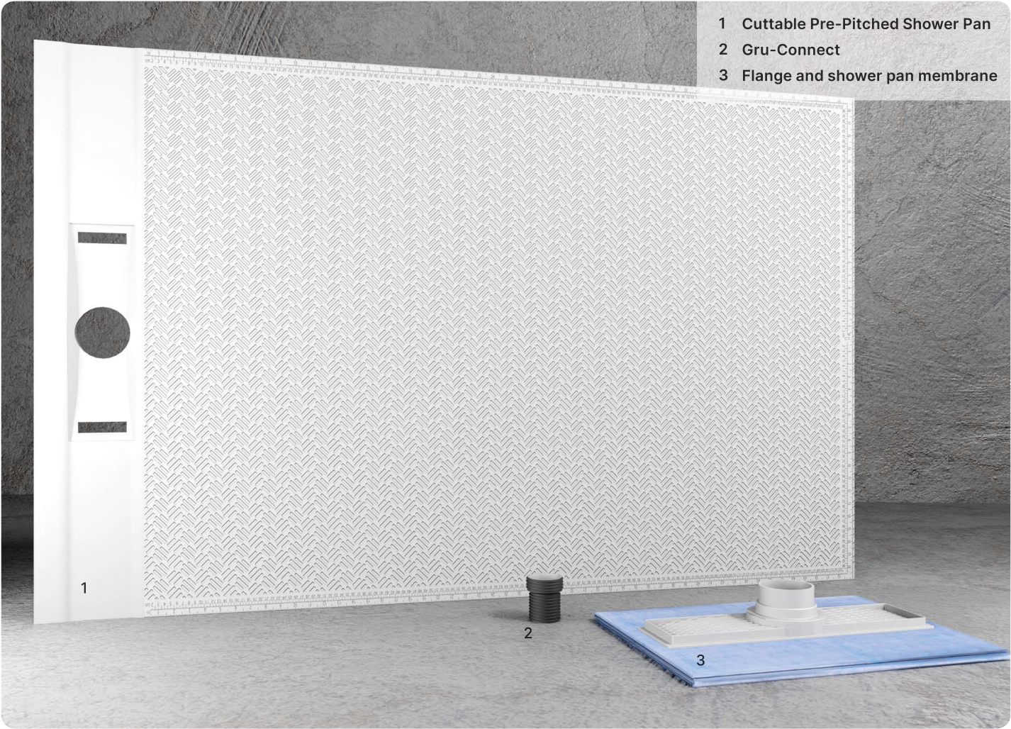
Waterproofing Membrane
